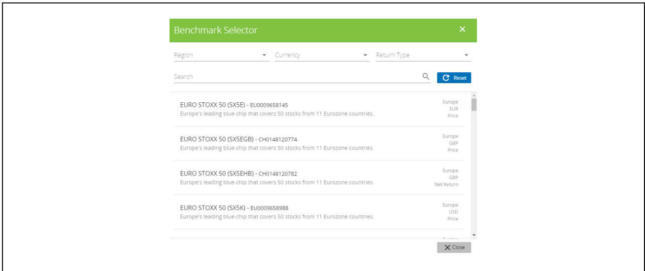
Figure 4-3. Benchmark Selector
