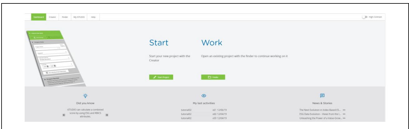
Figure 2-1. Dashboard page
