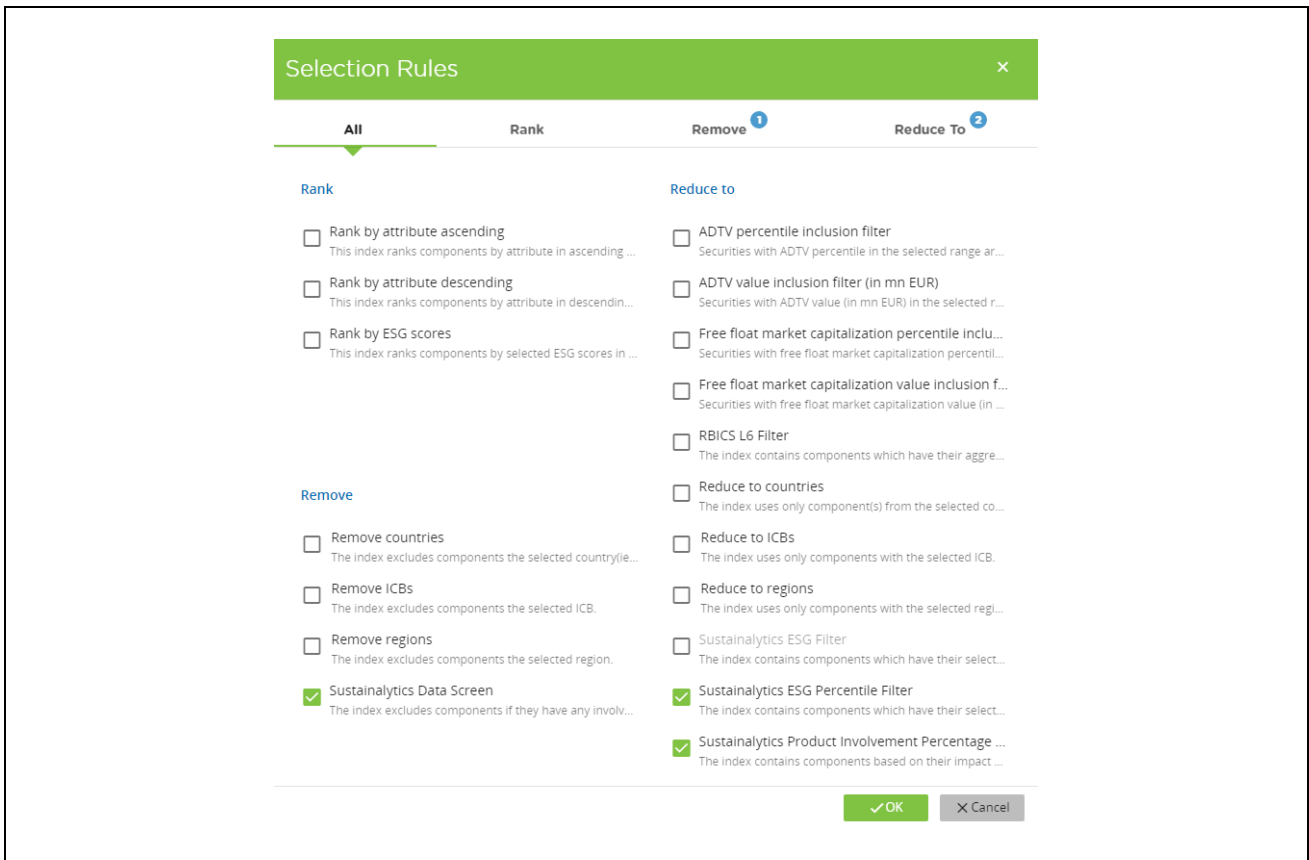
Figure 3-7. Selection Rules
