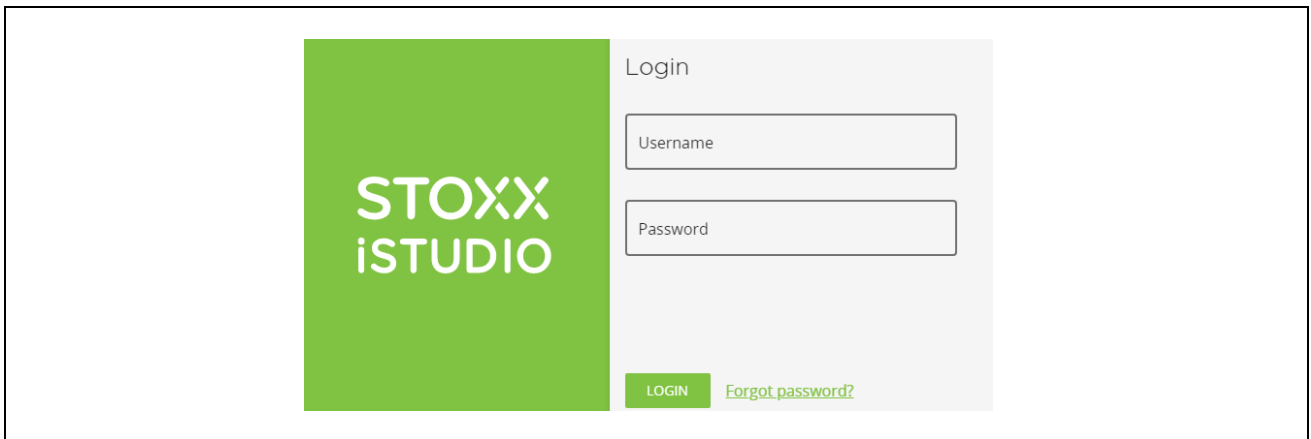
Figure 1-1. Login page
