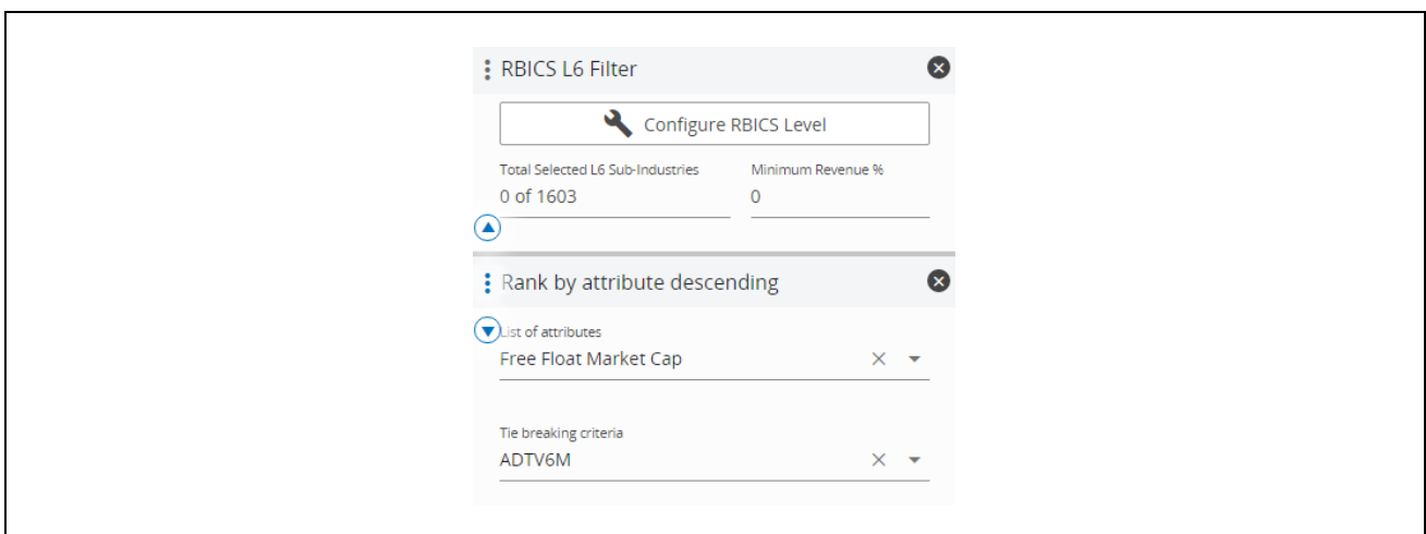
Figure 3-8. Selected rules
