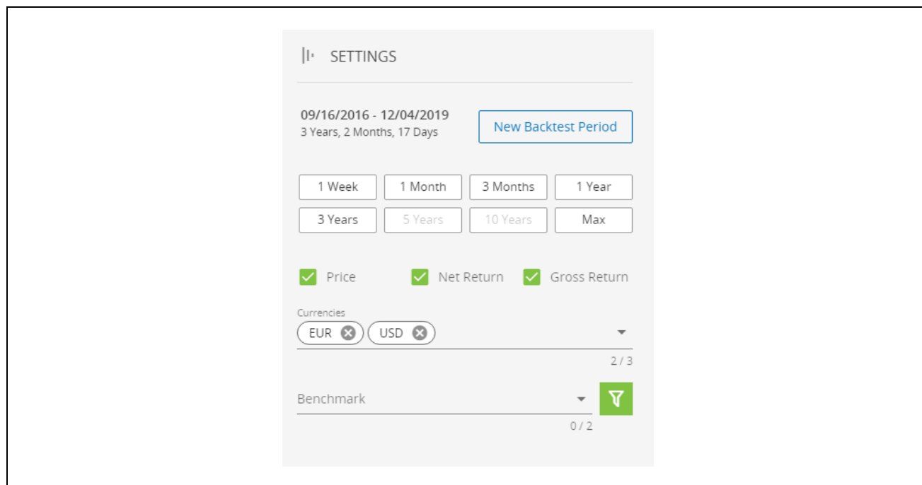
Figure 4-2. Settings
